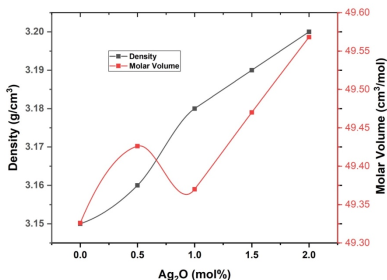
Fig. 1. Variation in the glass density and molar volume versus the doped Ag 2 O ratio. Density and molar volume.
