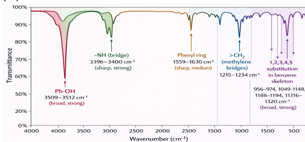
Fig. 3: FTIR Spectroscopic Characterization of 2, 4-DBAF Copolymer
