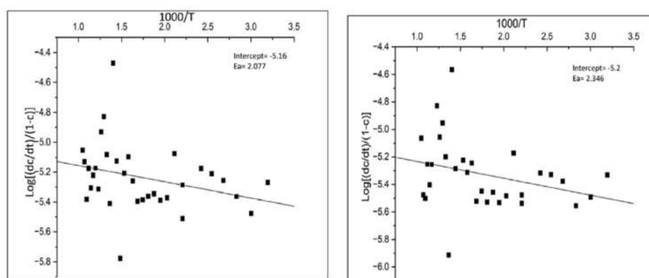
Fig8(a): Sharp–Wentworthplots of SATF-I-Cu (b) SATF-I-Ni
