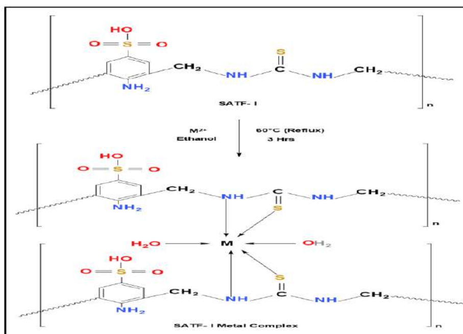
Fig. 1: Synthesis of SATF-I Metal complexes [M= Cu, Ni]
