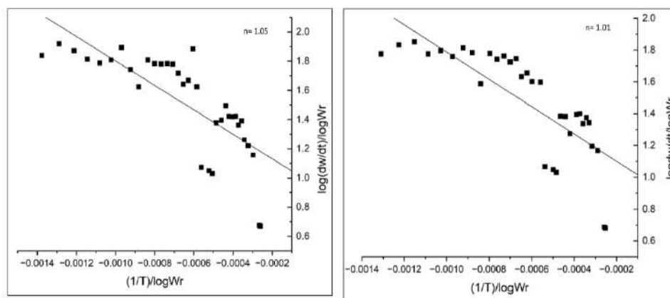
Fig9(a): Freeman-Carroll Plot of SATF-I-Cu (b) SATF-I-Ni
