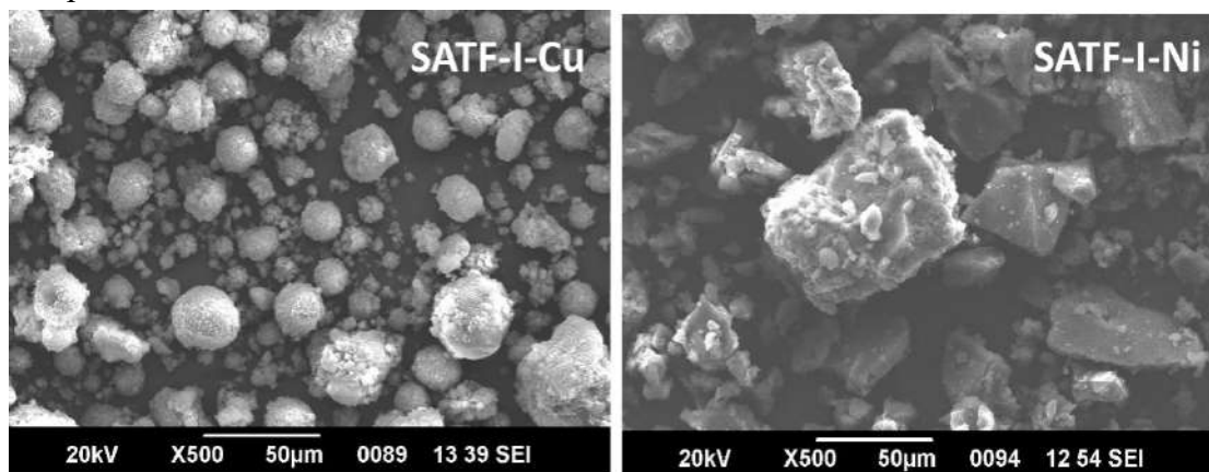
Fig. 5. SEM Micrographs of (a)SATF-I-Cu, (b)SATF-I-Ni
