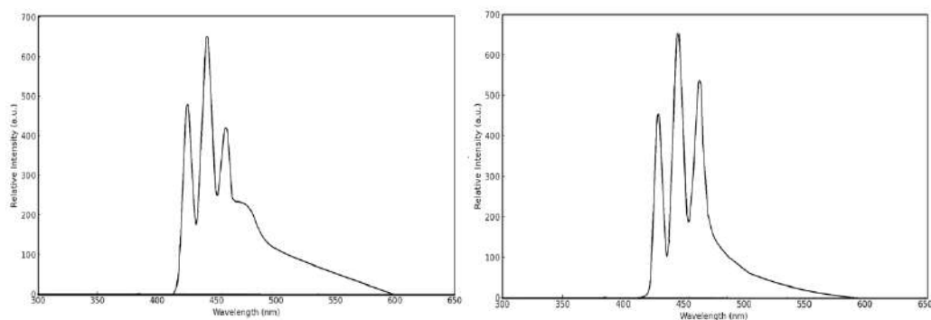
Fig.11:(a) PL Spectra SATF-I-Cu(b) SATF-I-Ni Complex
