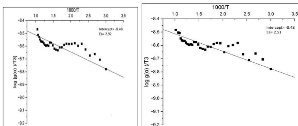
Fig10(a).Activation Energy ( E_a ) By Freeman-CarrollPlot of (a)SATF-I-Cu(b)SATF-I-NiComplexes
