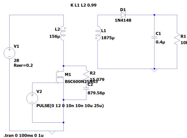
Figure 4. Flyback converter simulation circuit
