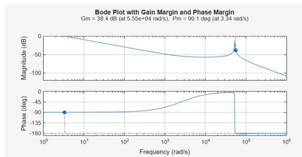
Figure 6. Bode plot of the system showing gain margin and phase margin obtained using MATLAB
