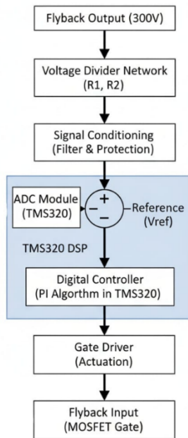
Figure 1. Block Diagram of the Closed loop system
