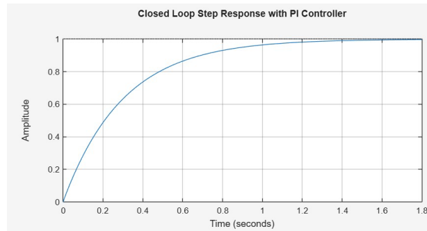
Figure 7. Step response derived from the MATLAB Simulation
