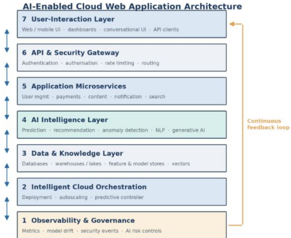
Figure 1.1 Conceptual architecture of the AI-enabled cloud web application, showing the seven layers and the continuous feedback loop.
